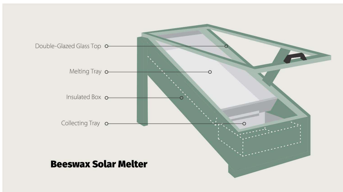
Figure 8. Solar Beeswax Melter Scheme
