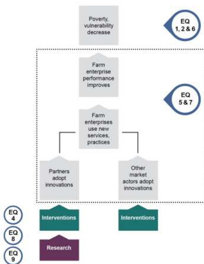
Figure 6: EQ Cluster 2
