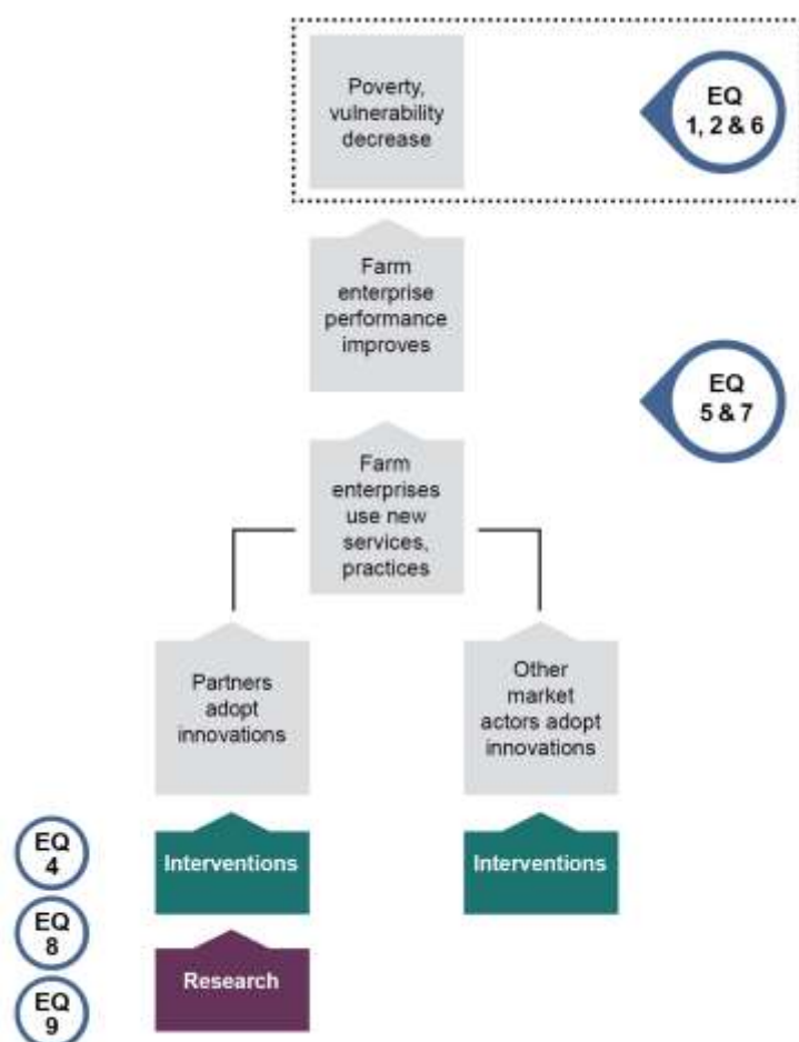
Figure 5: EQ Cluster 1
